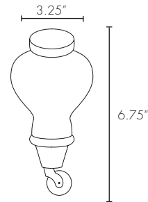
Wood Caster
